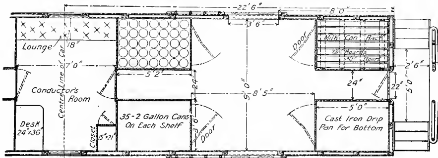
Fig. 273. Plan of Floor.
